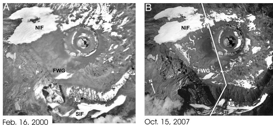
Fig. 1. Aerial photographs of the ice fields atop Kilimanjaro on February 16, 2000 (A) and October 15, 2007 (B). Note that two photos are required to cover the area in 2007 as emphasized by the white gap. Both images come from unrectified photos in which tilt and relief displacements have not been removed, thus possibly giving false impressions of the relative sizes of features. Both glaciers and snow cover appear in these images and cannot be distinguished at this reduced scale ( \approx 1:100,000 ).
